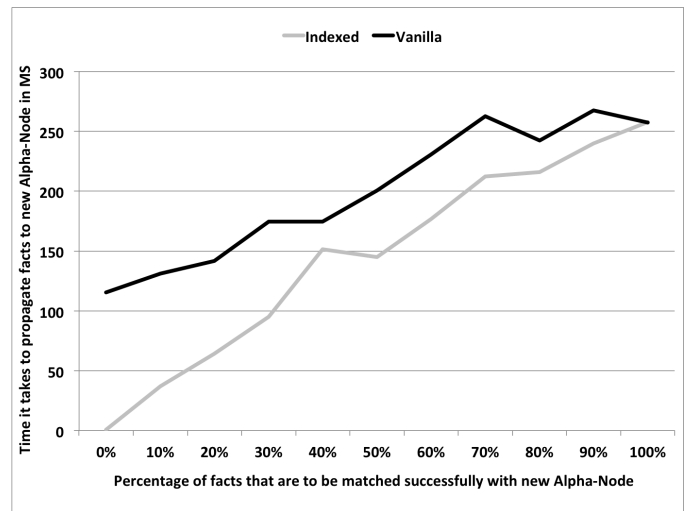
Figure 4: A comparison of the propagation of the working memory to the new Alpha-node of our extension and Drools with a varying percentage of facts that successfully match the new Alpha-node.
