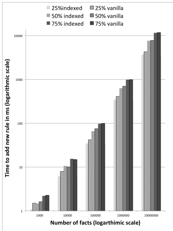
Figure 3: A comparison of the runtime of our extension and Drools with a varying number of facts in the working memory.
