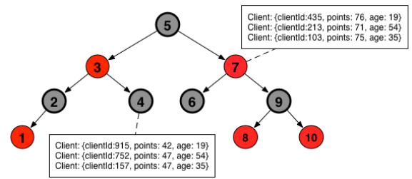
Figure 2: An example of a Red-black tree.
