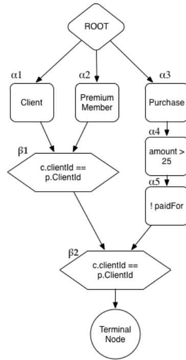
Figure 1: An example of a simple RETE-network.
