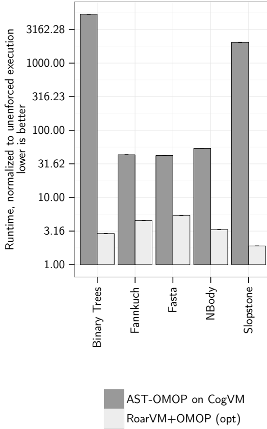
Figure 8.6.: Enforcement Overhead, logarithmic scale: Comparing unenforced execution of kernel benchmarks with enforced execution on RoarVM+OMOP (opt) and CogVM with AST-OMOP. The reified operations implement the standard semantics and on the RoarVM+OMOP (opt) lead to an average overhead of 3.4x (min 1.9x, max 5.4x). On the CogVM with the AST-OMOP, this overhead is on average 254.4x (min 42.1x, max 5346.0x).
