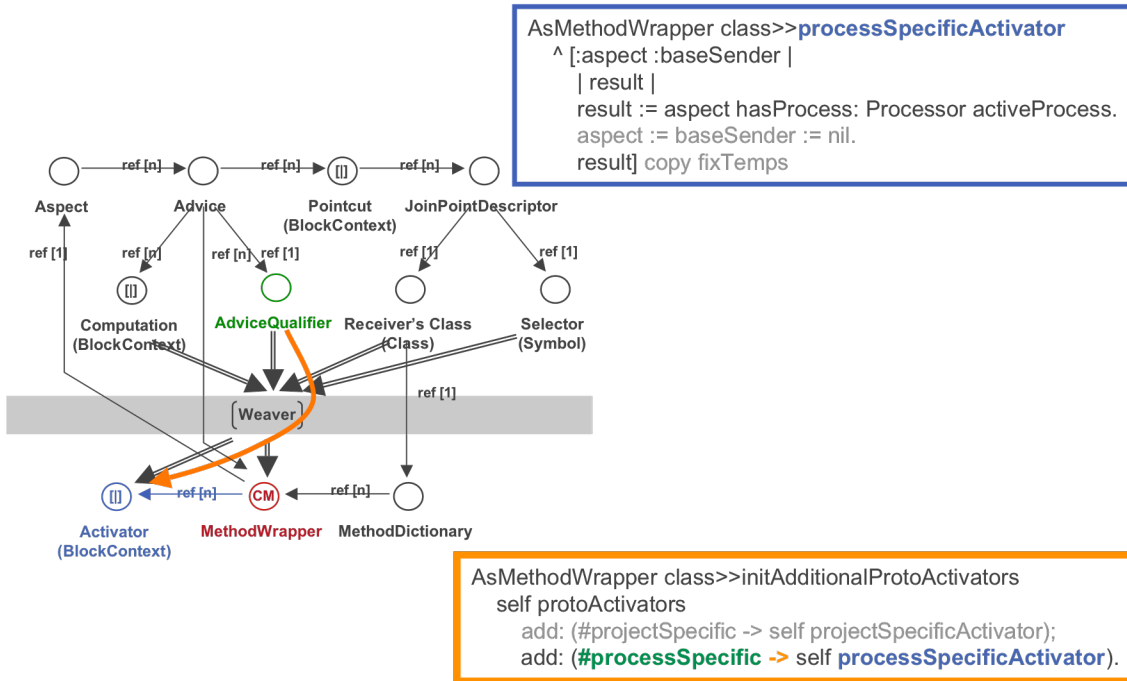
Figure 1: All that is necessary to enable process-specific advice activation
