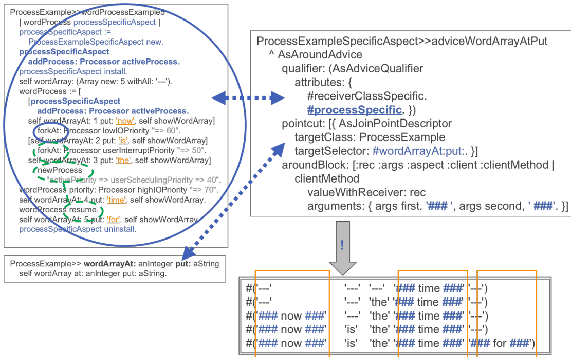
Figure 2: Instrumentation and effect of ProcessExample>>wordArrayAt:
